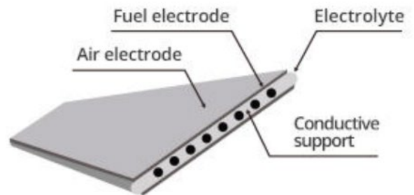
SOFC cell structure
